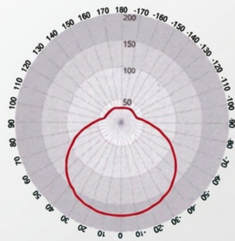
Emitter WITH reflector Emitter WITH reflector
